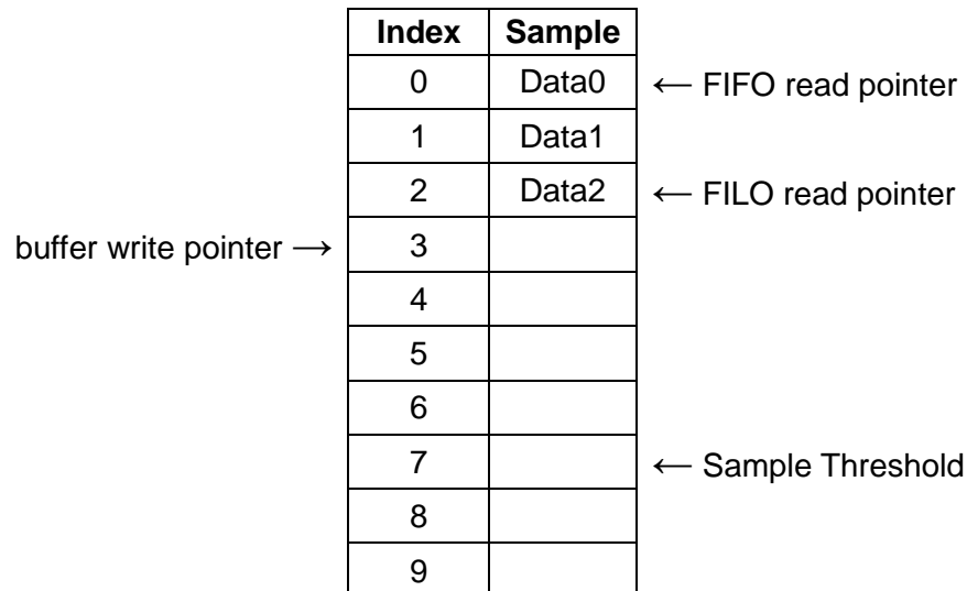
Figure 10. Buffer Filling
